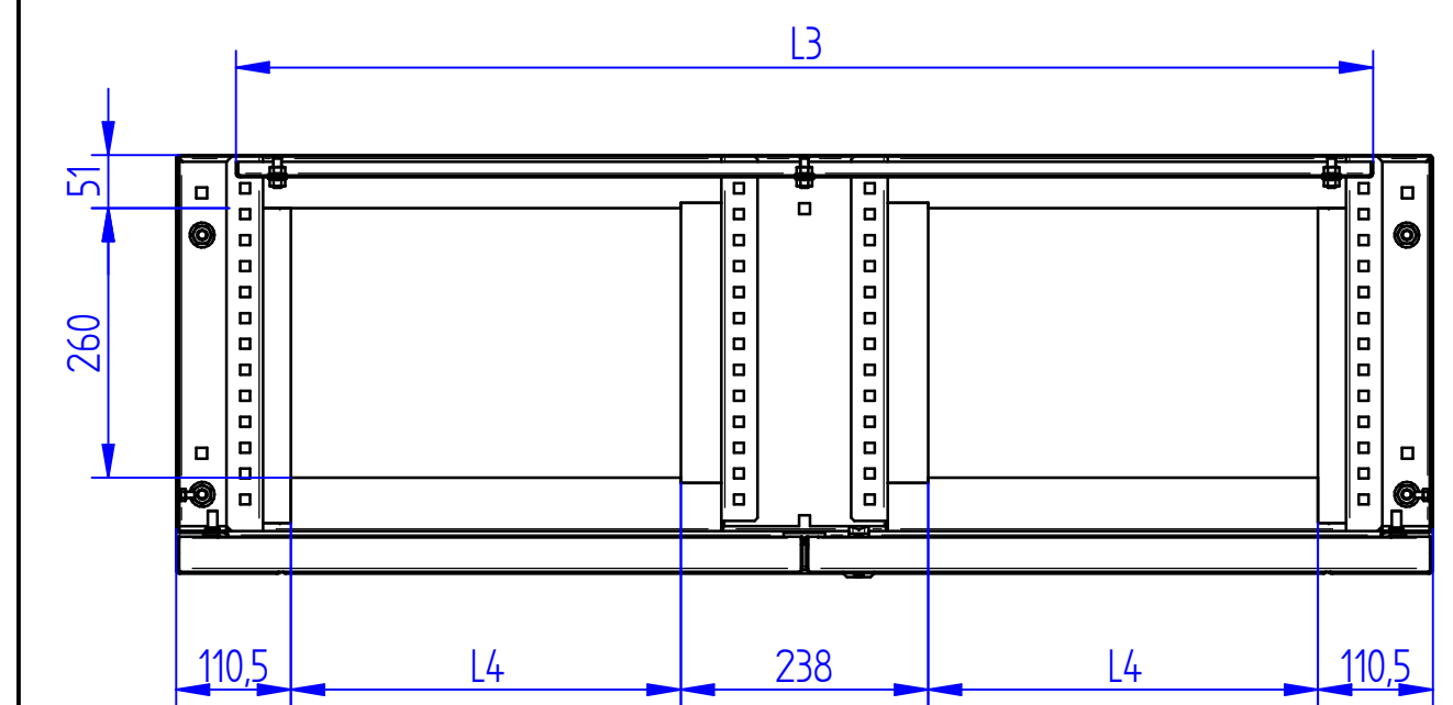
SECTION C-C
