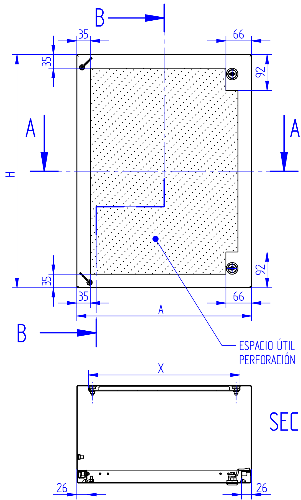
VISTA FRONTAL
